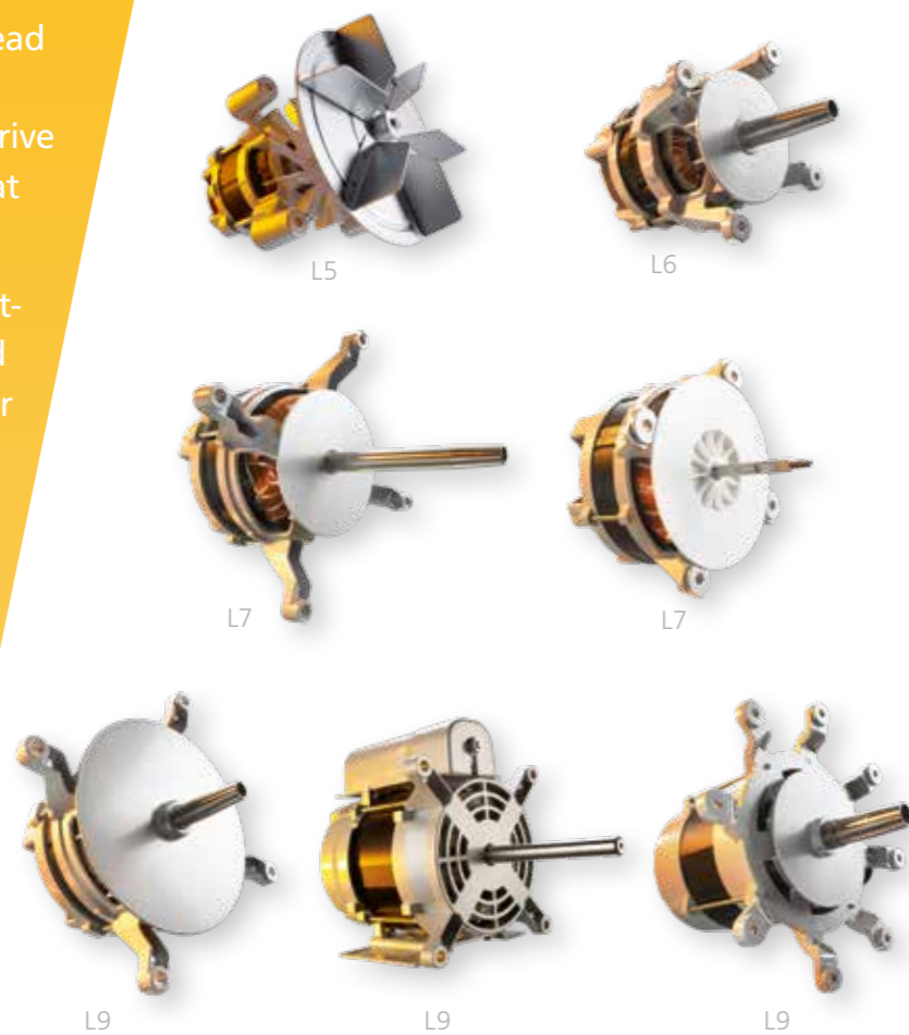
Various customized versions sizes L5 to L9 and SYL4 to SYL11.
